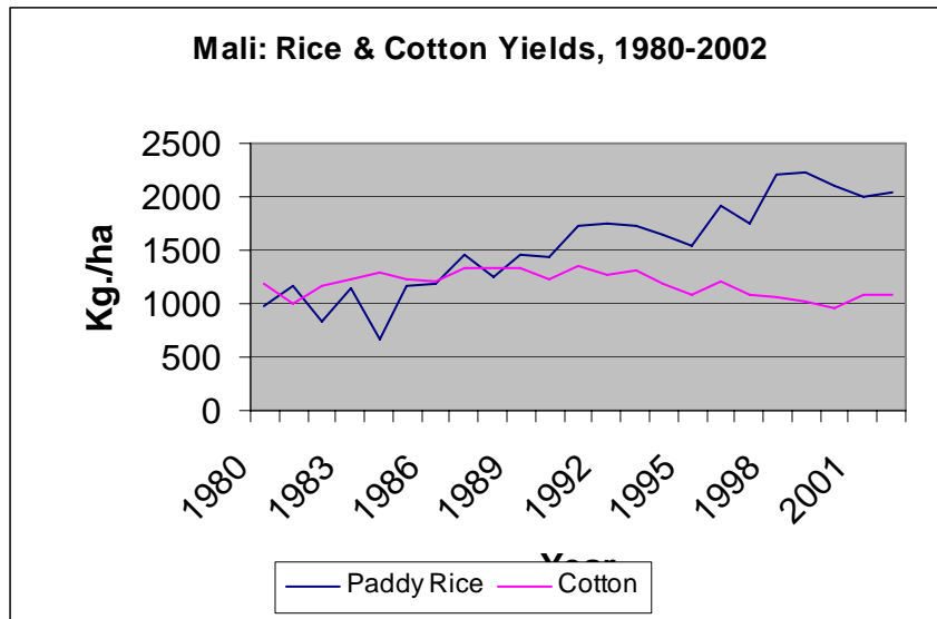
Figure 3.3.1 Rice and Cotton Yields (1980-2002)
